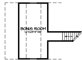
BONUS ROOM PLAN A-3
