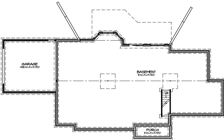
FOUNDATION PLAN A-2
