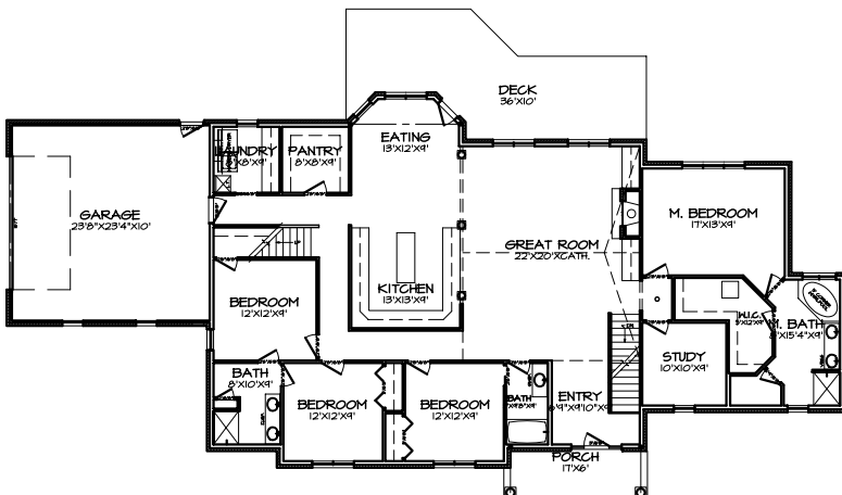
FIRST FLOOR PLAN A-3
